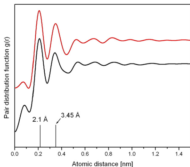
Fig. 4. Pair distribution functions (PDFs) calculated from two SAED patterns obtained from FeS am . The two peaks at ~2.1 and 3.45 Å are consistent with Fe-S and S-S distances in [FeS 4 ] tetrahedra, respectively.
