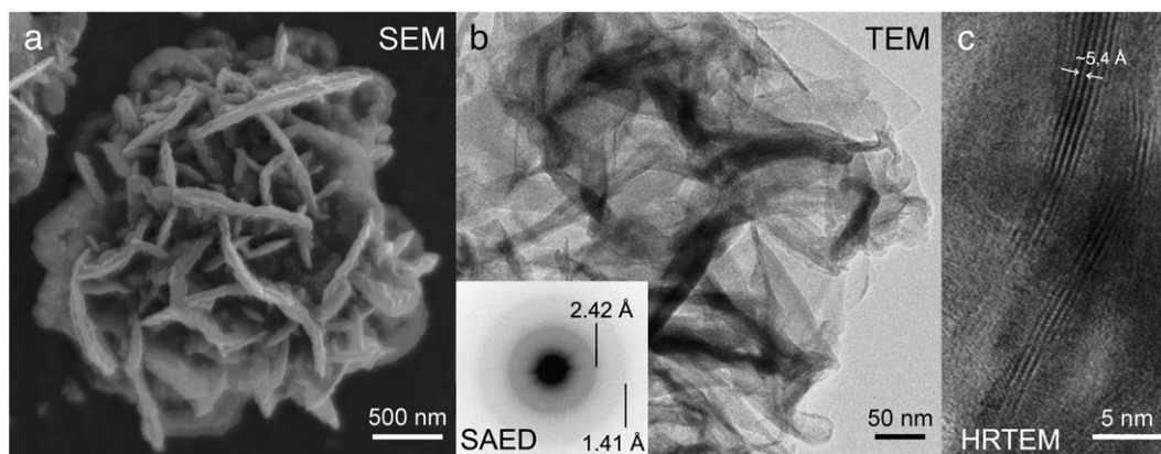
Fig. 3. (a) SEM, (b) bright-field TEM, and (c) HRTEM images of FeS am (UP). The inset in the lower left of b is a SAED pattern obtained from an aggregate similar to that shown in b, and its diffuse rings indicate a poorly crystalline character of the material. The measured d-spacing between atomic layers in c is 5.4 Å, substantially larger than that expected for crystalline mackinawite (5.03 Å).
