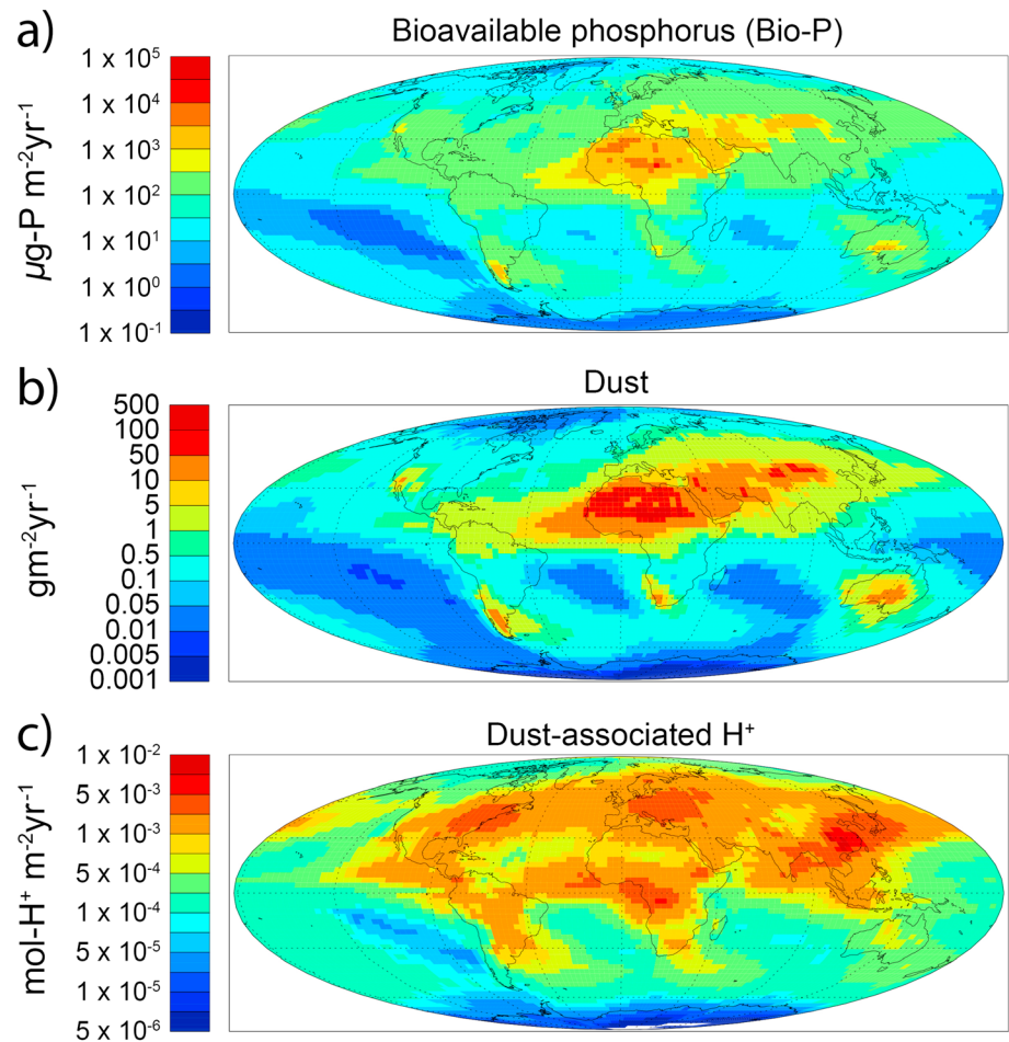
Figure 2. Annual deposition rate of (a) bioavailable phosphorus in \mu\text{g-P m}^{-2}\text{yr}^{-1} , (b) dust in \text{g/m}^2/\text{year} , and (c) dust-associated \text{H}^+ ions in \text{mol-H}^+ \text{m}^{-2}\text{yr}^{-1} .
