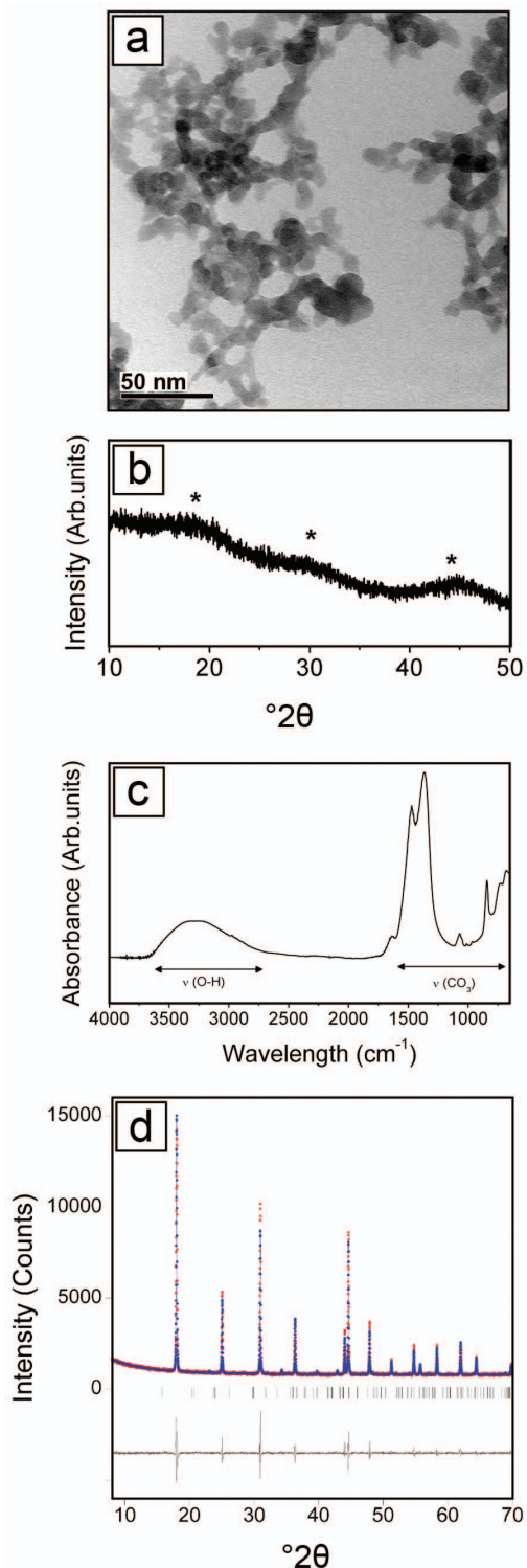
FIG. 2. (a) TEM image of the initial precursor showing spherical nanoparticles with diameters of between 10 and 20 nm; (b) XRD pattern of the gel-like precursor showing its amorphous character; (c) FTIR profile of the precursor showing bands corresponding to water and carbonate vibrations; and (d) pattern-matching refinement of the XRD pattern of the final end product indexed as hexagonal \text{NdCO}_3(\text{OH}) .
